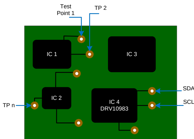
Figure 15. Example Circuit for Bed of Nails Tester
