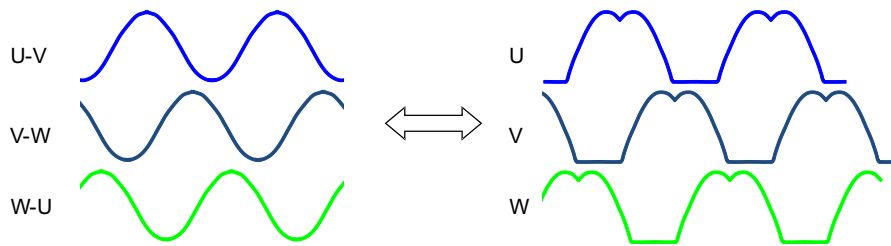
Sinusoidal voltage from phase to phase
