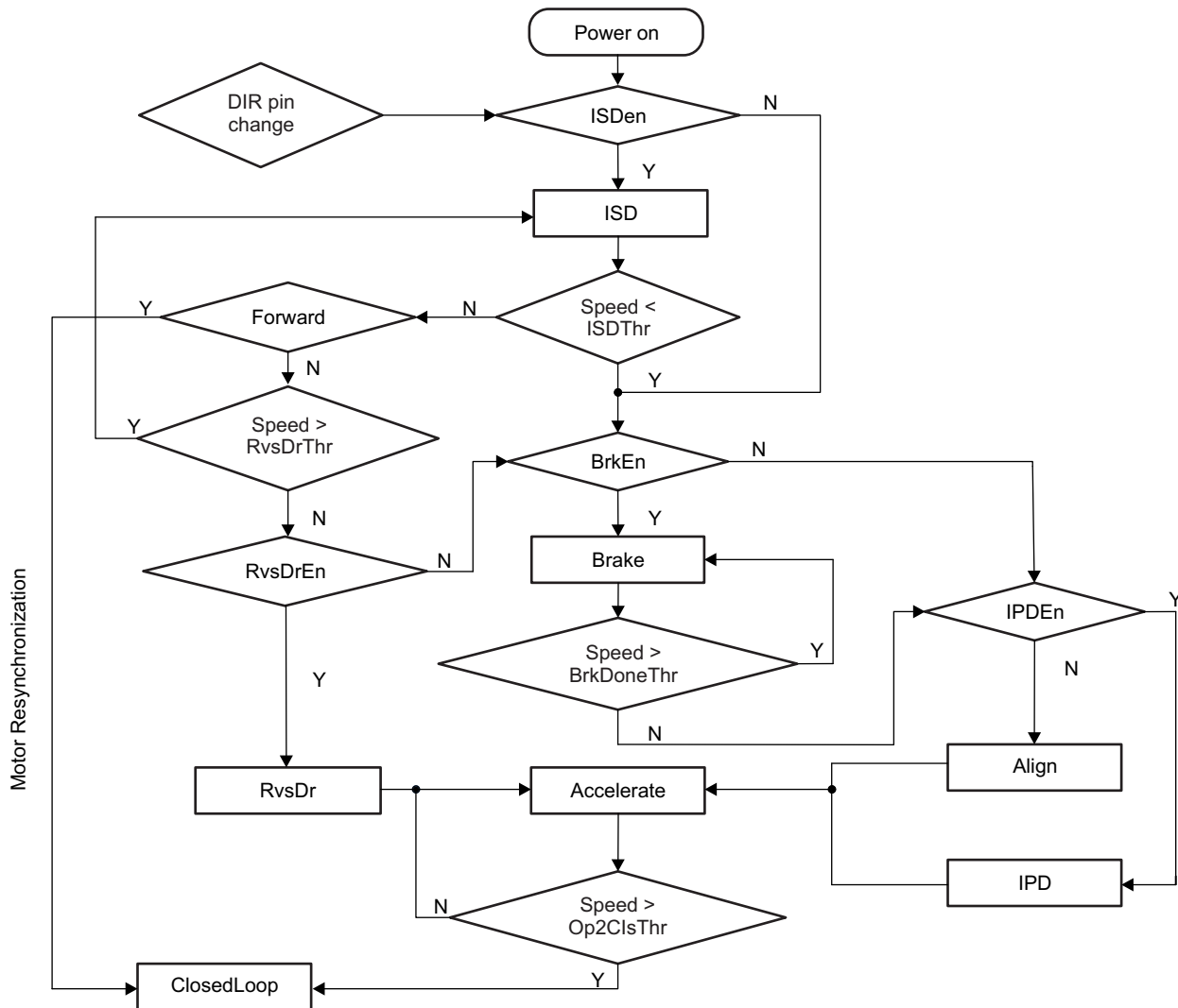
Figure 9. Motor Starting-Up Flow
