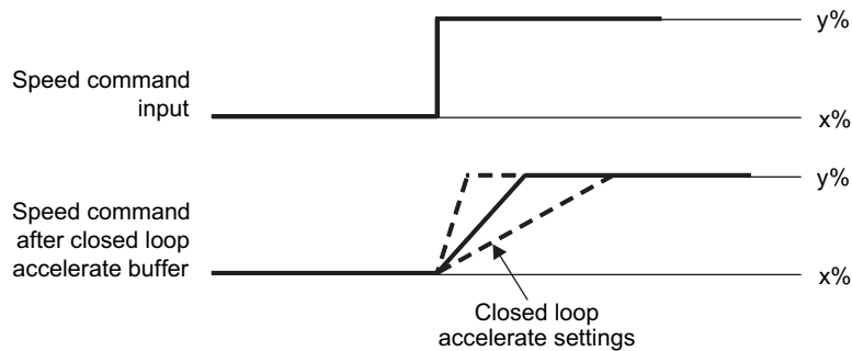
Figure 23. Closed Loop Accelerate
