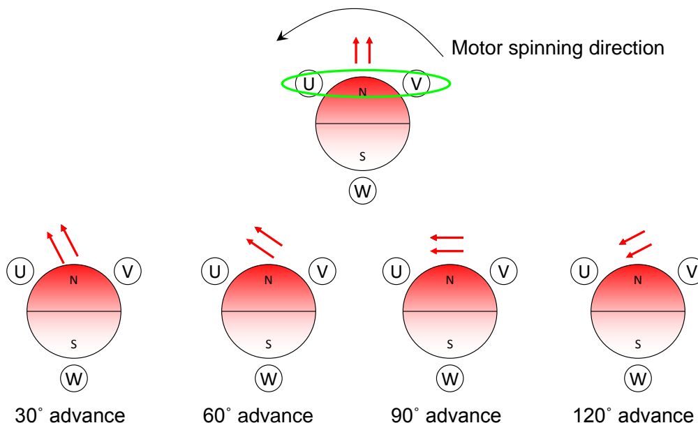
Figure 15. IPD Advance Angle
