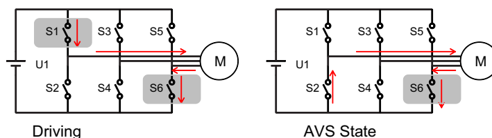
Figure 34. Inductive AVS
