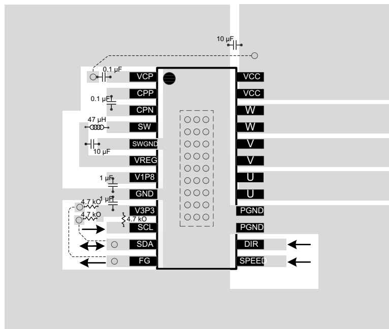
Figure 42. Layout Schematic
