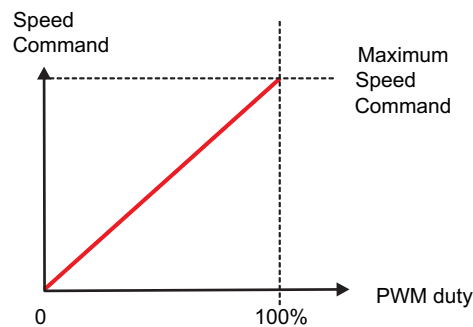
Figure 21. PWM Mode Speed Command
