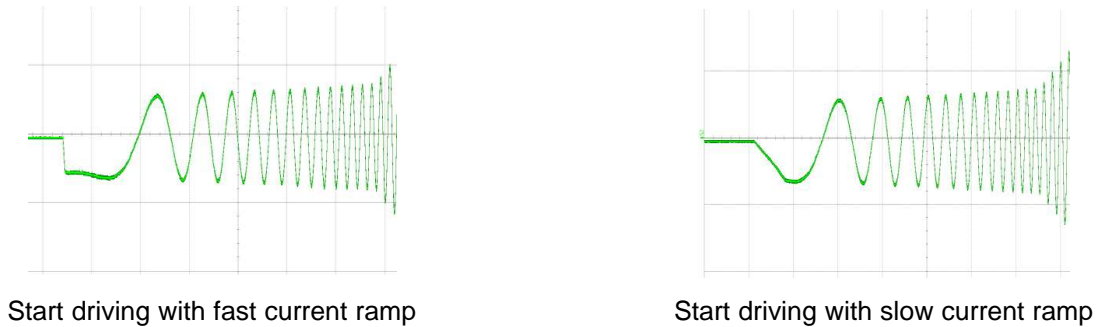
Figure 18. Motor Startup Current Ramp
