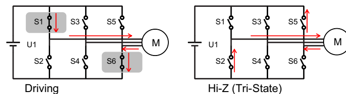
Figure 14. IPD Release Mode 1
