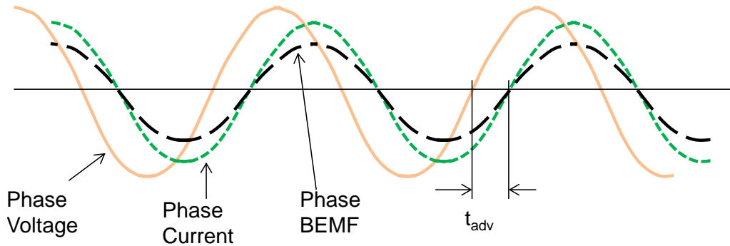
Figure 24. Advance Time ( t_{adv} ) Definition
