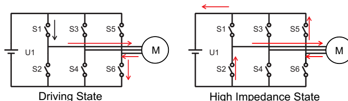
Figure 33. Inductive Mode Voltage Surge
