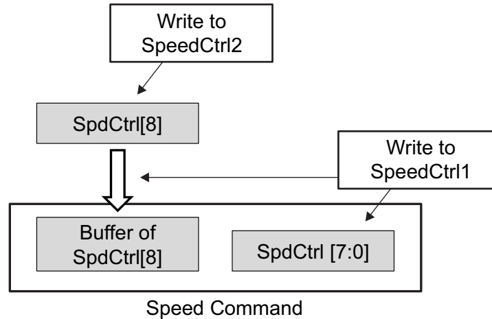
Figure 22. I 2 C Mode Speed Control
