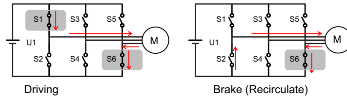
Figure 13. IPD Release Mode 0
