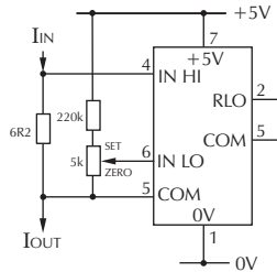
Measuring 4-20mA to read 0-999.
