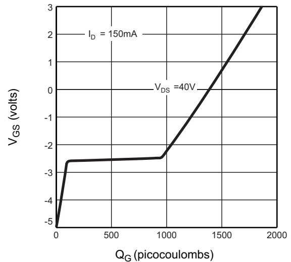
Gate Drive Dynamic Characteristics
