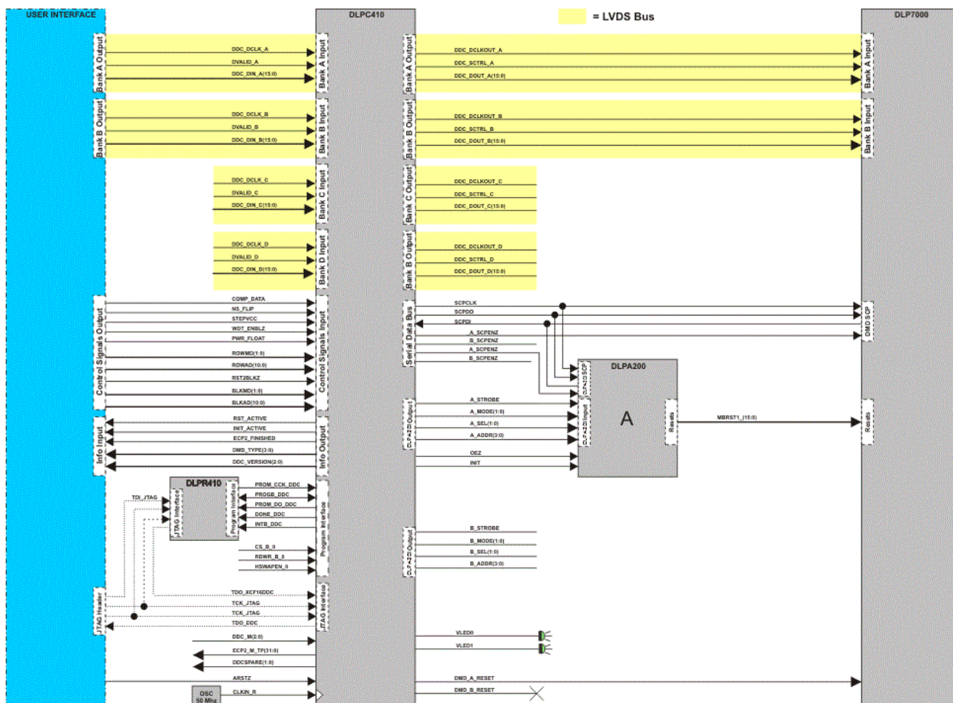
Figure 8. DLPC410 and DLP7000 Chipset Block Diagram
