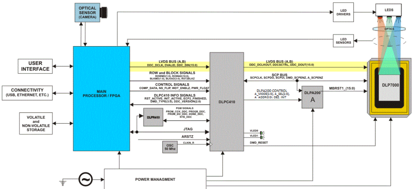
Figure 19. DLPC410 and DLP7000 Embedded Example Block Diagram
