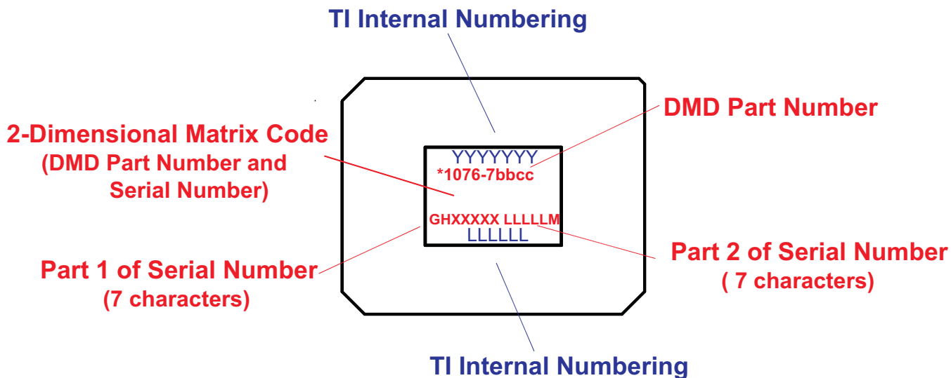
Figure 22. Device Marking
