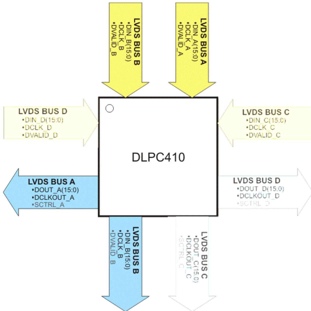
Figure 9. DLPC410 Data Flow
