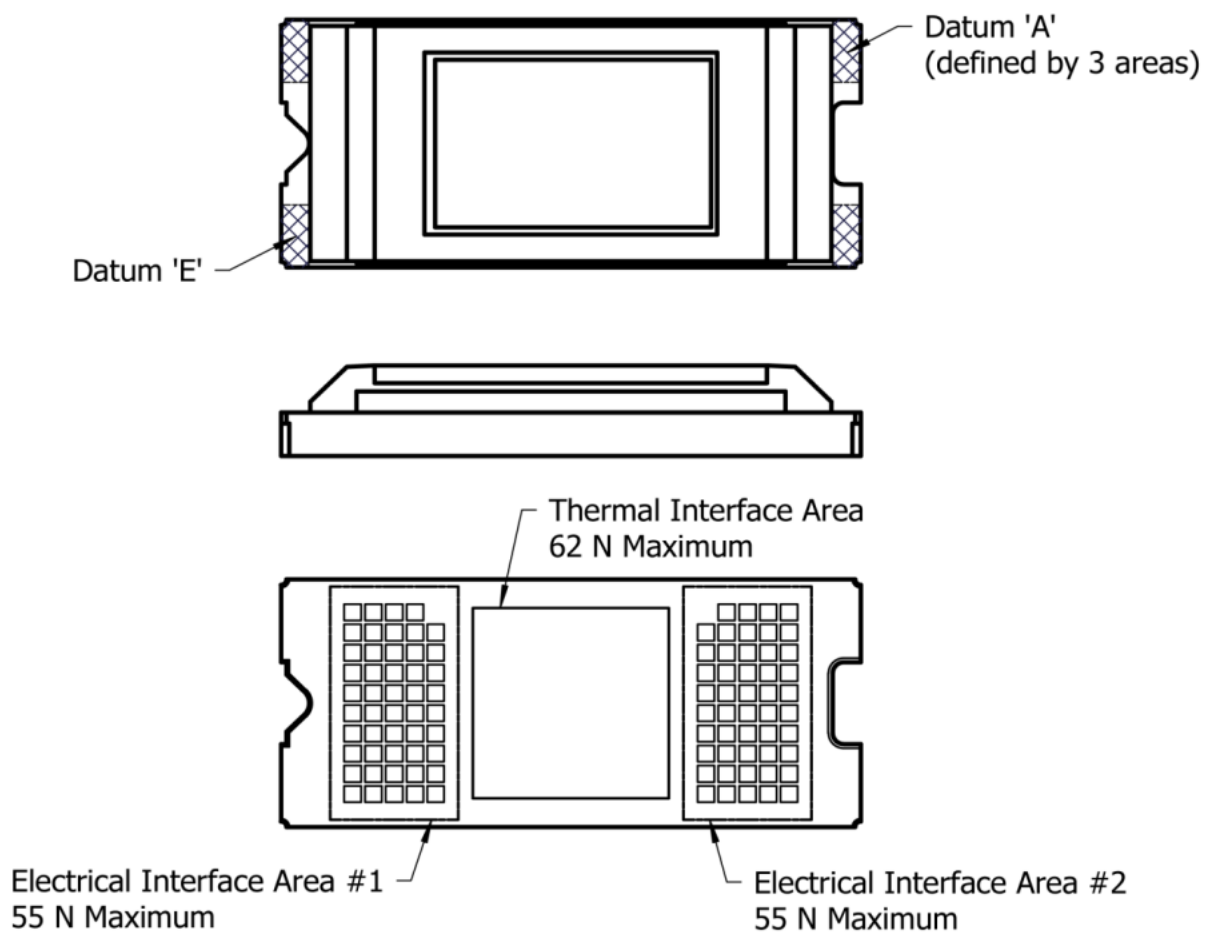
Figure 11. System Interface Loads for FQD
