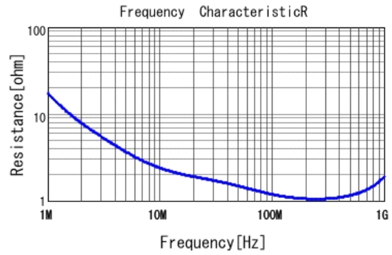
■ DK1B3EA221K86RAH01 R DCOV, 20degC
