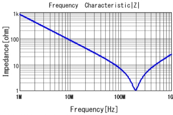
■ DK1B3EA221K86RAH01 |Z| DCOV, 20degC
