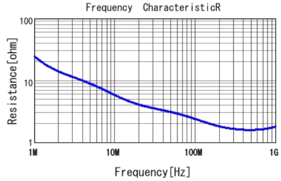
■ DK1B3EA101K86RBH01 R DCOV, 20degC
