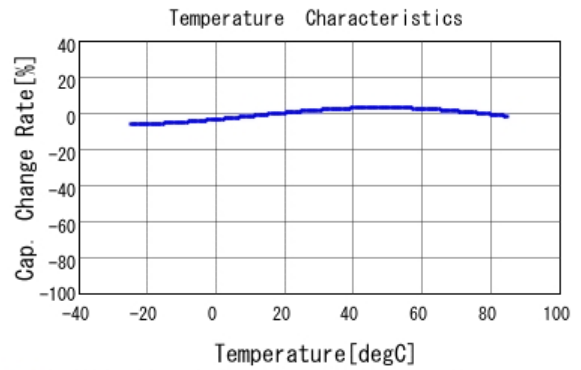
■ DK1B3EA101K86RBH01 C-Temp. capchange, DCOV, AC1Vrms
