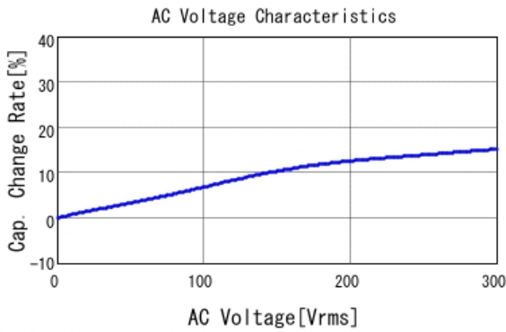
■ DK1B3EA101K86RBH01 C-AC Voltage capchange, DCOV, 20.0
