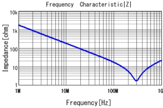
■ DK1B3EA101K86RBH01 |Z| DCOV, 20degC
