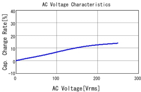
■ DK1B3EA101K86RAH01 C-AC Voltage capchange, DCOV, 20.0
