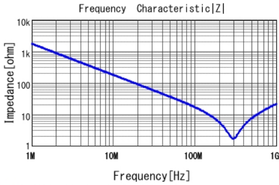
■ DK1B3EA101K86RAH01 |Z| DCOV, 20degC
