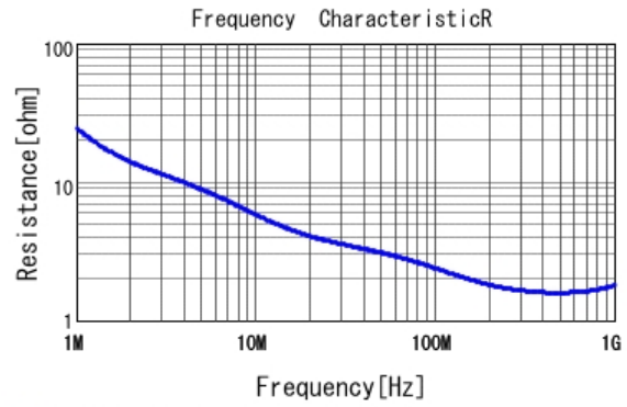
■ DK1B3EA101K86RAH01 R DCOV, 20degC
