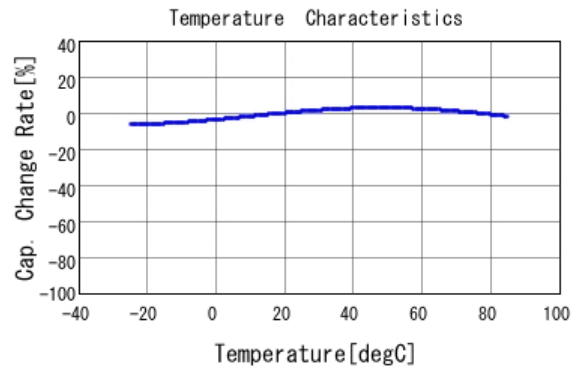
■ DK1B3EA101K86RAH01 C-Temp. capchange, DCOV, AC1Vrms
