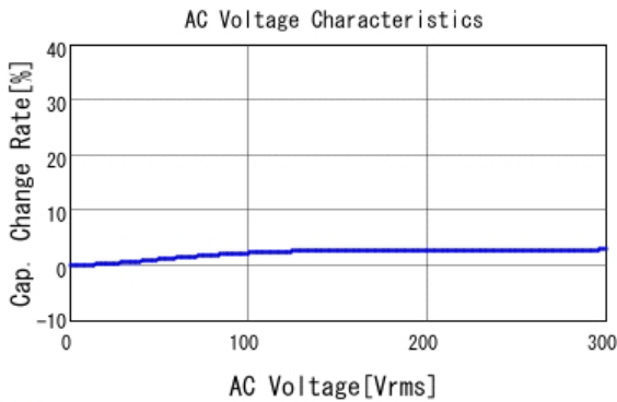
■ DK11XEA100K86RBH01 C-AC Voltage capchange, DCOV, 20.0
