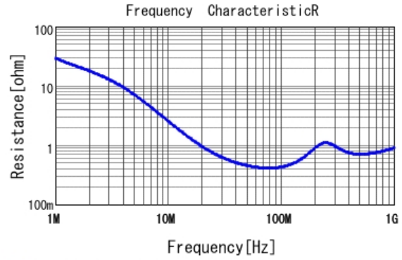
■ DK11XEA100K86RBH01 R DCOV, 20degC
