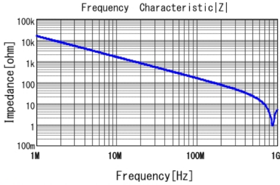
■ DK11XEA100K86RBH01 |Z| DCOV, 20degC
