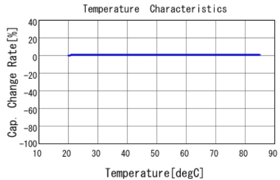
■ DK11XEA100K86RBH01 C-Temp. capchange, DCOV, AC1Vrms
