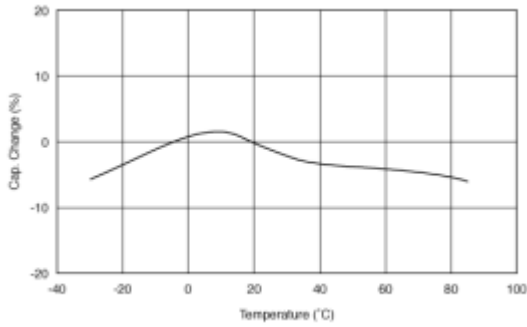
Capacitance - temperature characteristics
