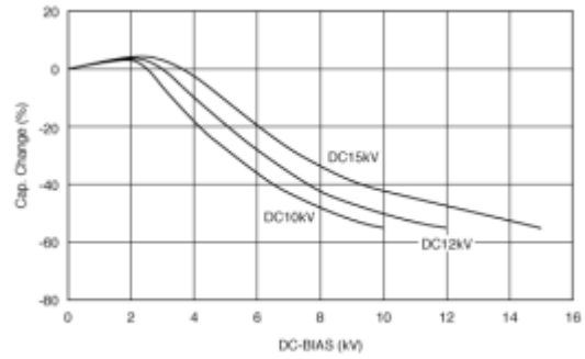
Capacitance - DC Bias Characteristics
