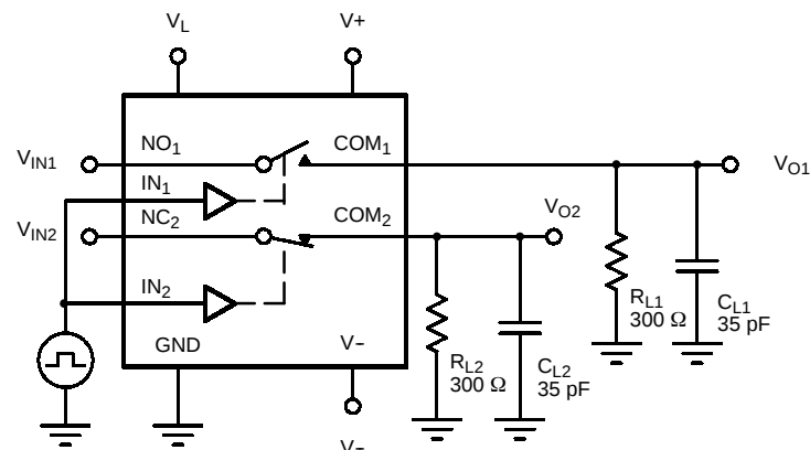
FIGURE 2. Switching Time
