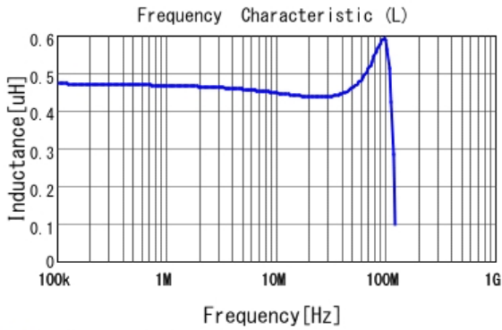
DFE2HCAHR47MJ0 L
