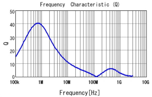
DFE2HCAHR47MJ0 Q
