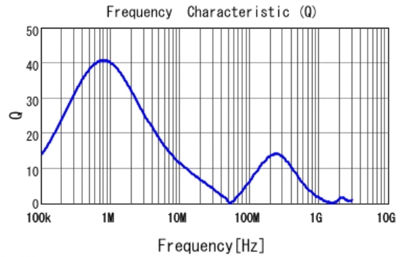
DFE2HCAH2R2MJ0 Q
