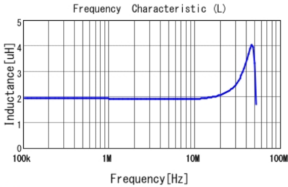
DFE2HCAH2R2MJ0 L
