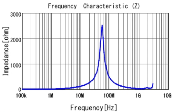
DFE2HCAH2R2MJ0 |Z|
