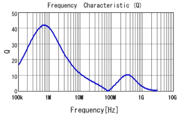
DFE2HCAH1R0MJ0 Q
