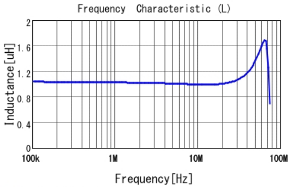
DFE2HCAH1R0MJ0 L
