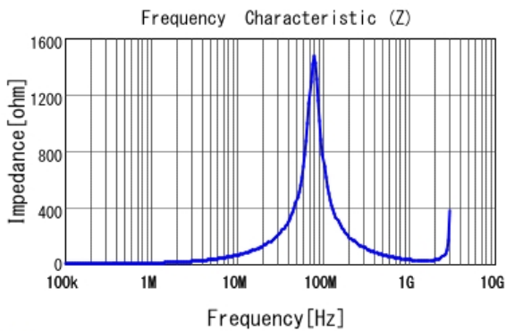
DFE2HCAH1R0MJ0 |Z|
