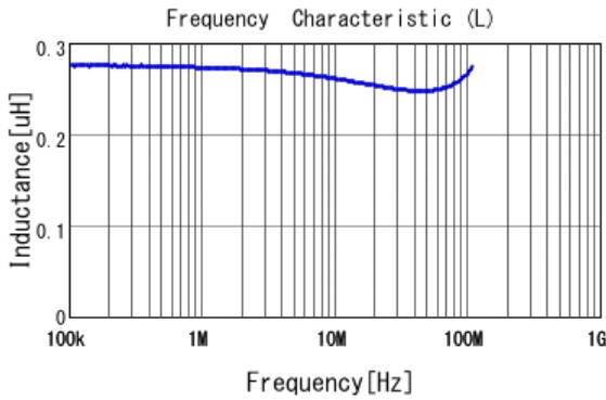
■ DFE18SANR24ME0 L
