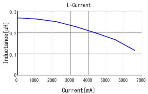
■ DFE18SANR24ME0 L-Current 20degC
