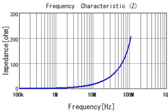
■ DFE18SANR24ME0 |Z|
