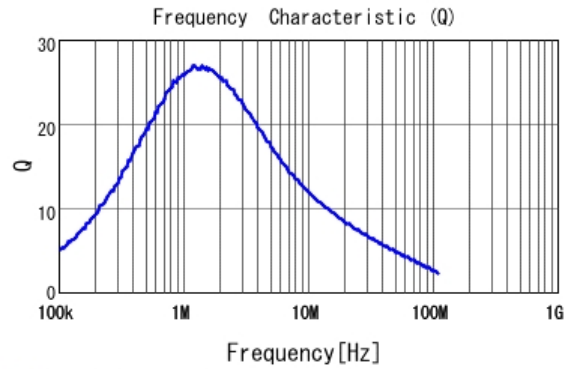
■ DFE18SANR24ME0 Q
