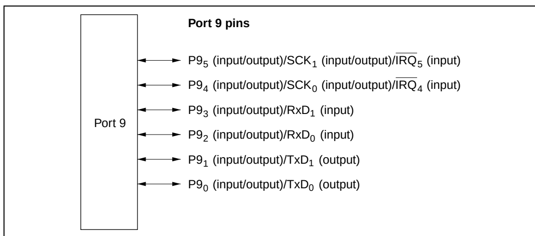
Figure 7.9 Port 9 Pin Configuration
