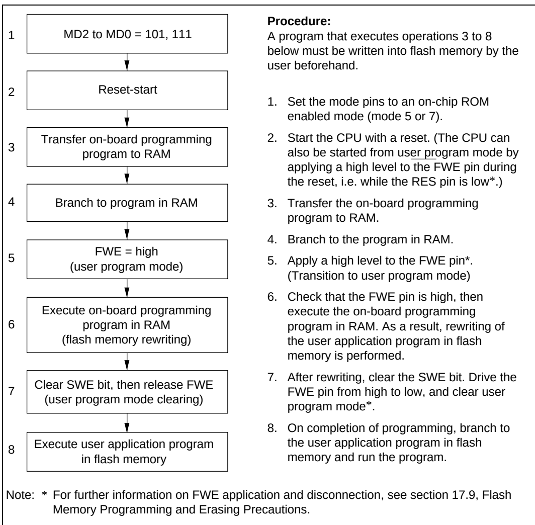
Figure 17.9 User Program Mode Execution Procedure (Example)
