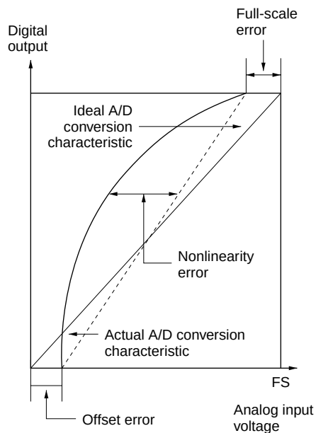
Figure 14.10 A/D Converter Accuracy Definitions (2)
