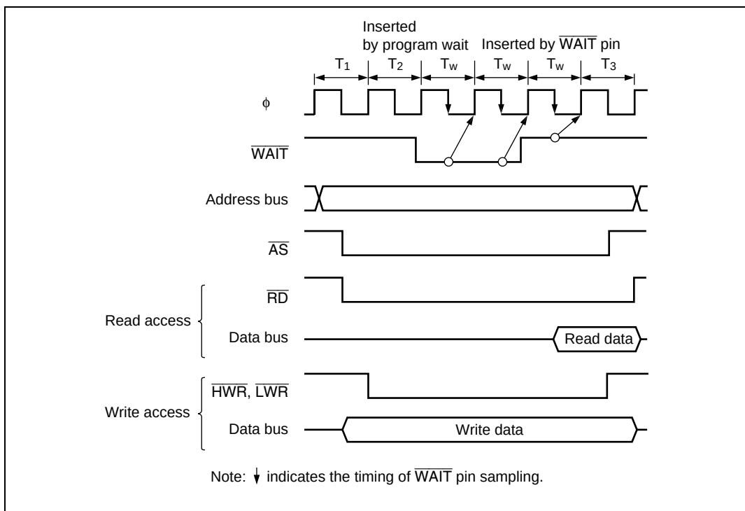
Figure 6.17 Example of Wait State Insertion Timing
