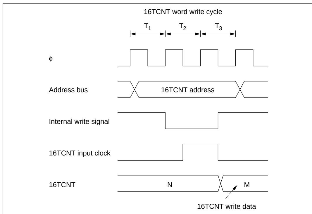
Figure 8.38 Contention between 16TCNT Word Write and Increment
