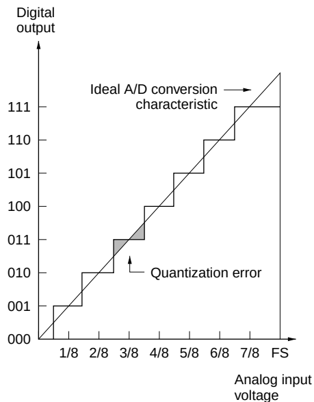
Figure 14.9 A/D Converter Accuracy Definitions (1)
