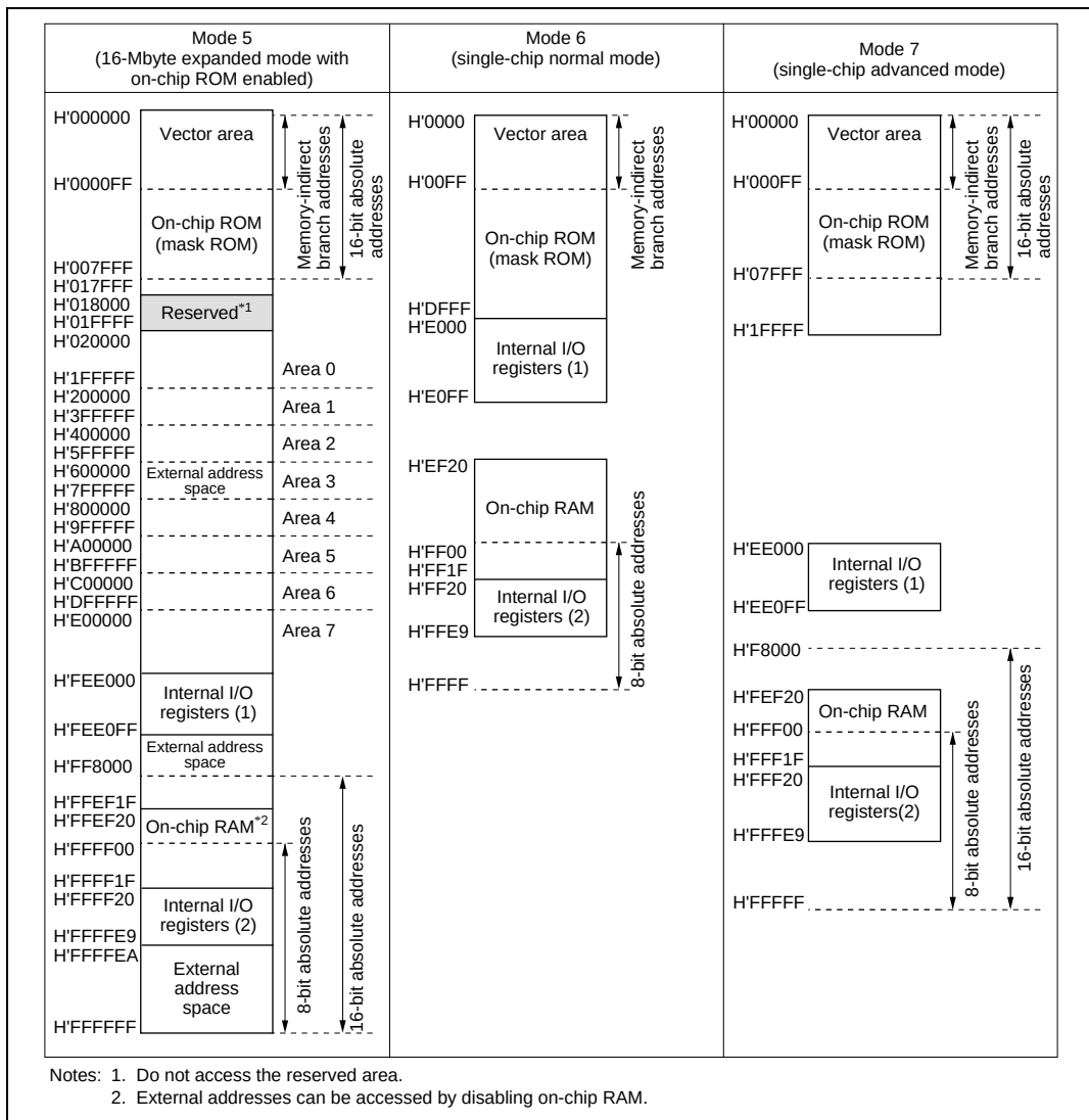
Figure 3.2 Memory Map of H8/3061 Masked ROM Version and H8/3061 Masked ROM B-Mask Version in Each Operating Mode (cont)
