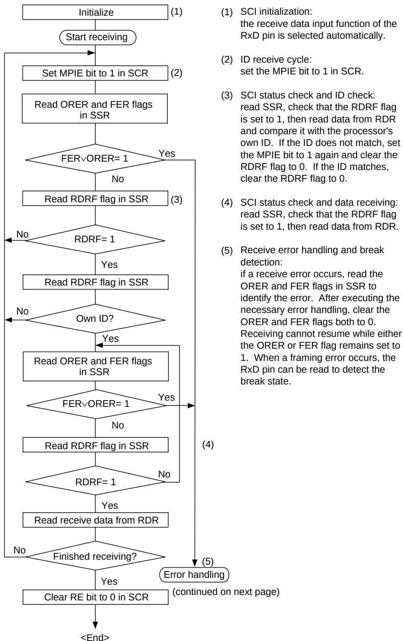
Figure 12.12 Sample Flowchart for Receiving Multiprocessor Serial Data
