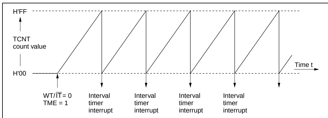
Figure 11.5 Interval Timer Operation
