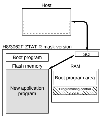
Figure 17.3 Boot Mode
