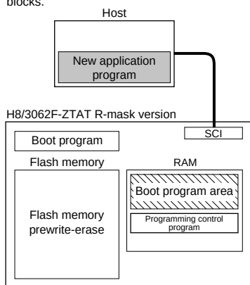
Figure 17.3 Boot Mode
