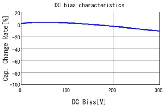
■ DE2F3KY103MA3BU02F C-DC bias capchange, 20.0degC, AC1
