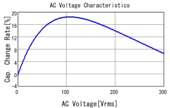
■ DE2F3KY103MA3BU02F C-AC Voltage capchange, DCOV, 20.0
