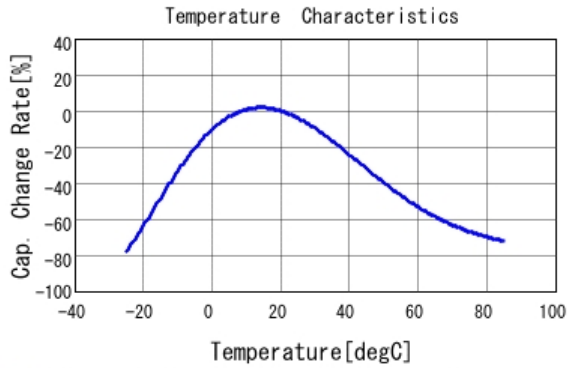
■ DE2F3KY103MA3BU02F C-Temp. capchange, DCOV, AC1Vrms
