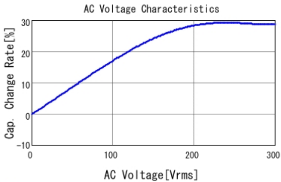
■ DE2E3SA472MA3BX02F C-AC Voltage capchange, DCOV, 20.0
