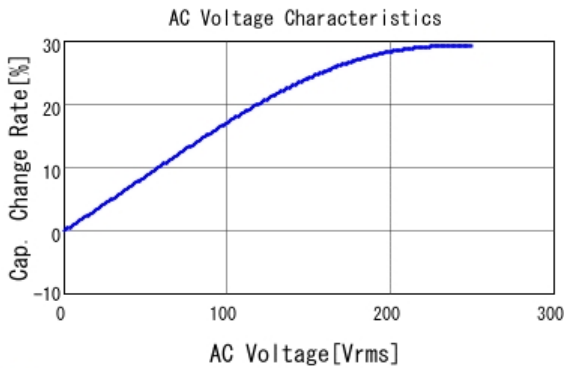
■ DE2E3SA472MA2BT01F C-AC Voltage capchange, DCOV, 20.0
