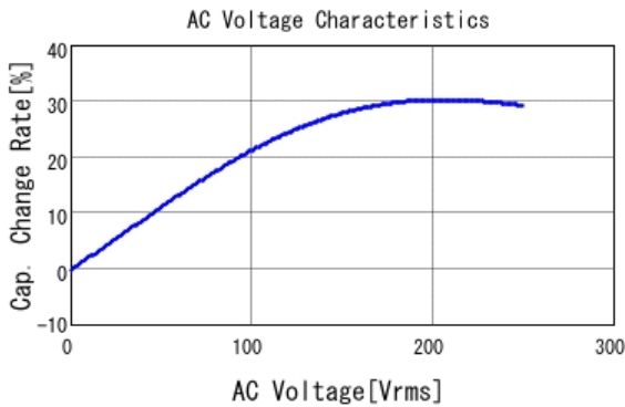
■ DE2E3SA222MJ3BT02F C-AC Voltage capchange, DCOV, 20.0
