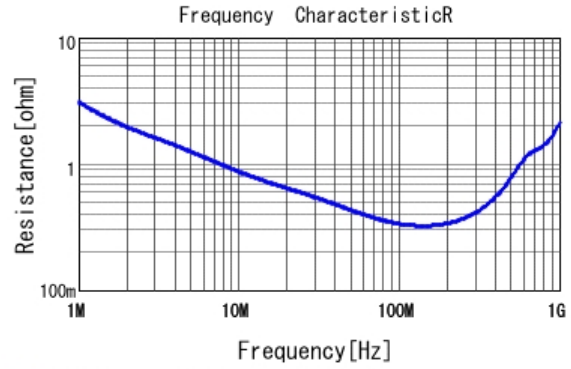
■ DE2E3SA152MA2BT01F R DCOV, 20degC
