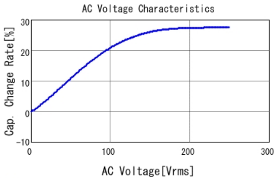
■ DE2E3SA152MA2BT01F C-AC Voltage capchange, DCOV, 20.0
