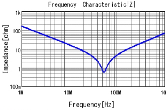
■ DE2E3SA102MN3AY02F |Z| DCOV, 20degC
