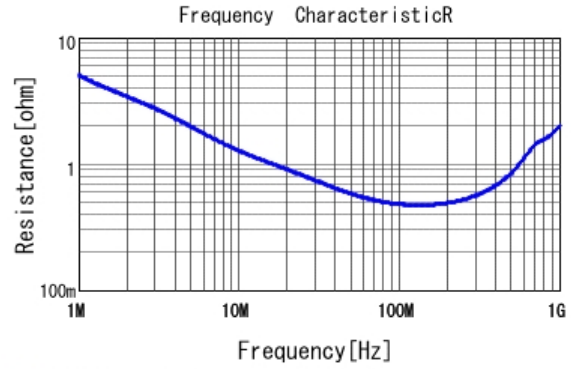
■ DE2E3SA102MN3AY02F R DCOV, 20degC
