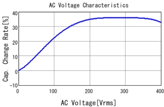
■ DE2E3SA102MN3AY02F C-AC Voltage capchange, DCOV, 20.0
