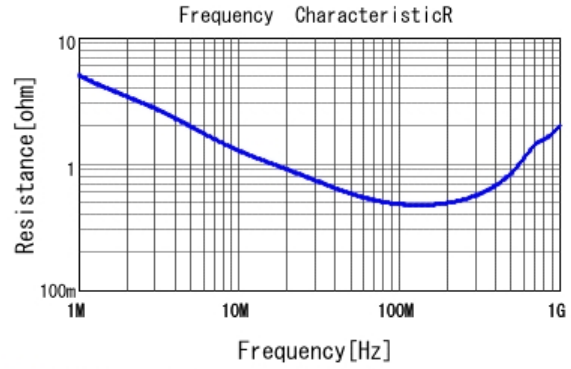
■ DE2E3SA102MA3BY02F R DCOV, 20degC
