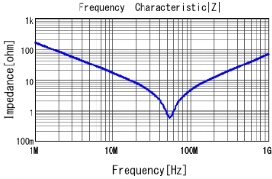
■ DE2E3SA102MA3BY02F |Z| DCOV, 20degC
