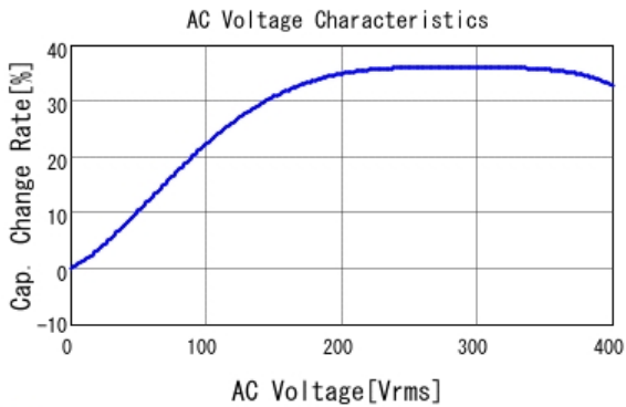
■ DE2E3SA102MA3BY02F C-AC Voltage capchange, DCOV, 20.0
