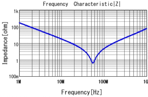
■ DE2E3SA102MA3BT02F |Z| DCOV, 20degC
