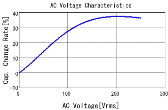
■ DE2E3SA102MA3BT02F C-AC Voltage capchange, DCOV, 20.0
