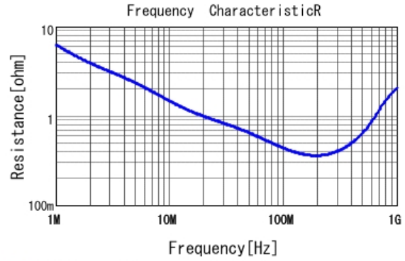
■ DE2E3SA102MA3BT02F R DCOV, 20degC
