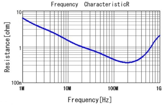
■ DE2E3SA102MA2BT01F R DCOV, 20degC
