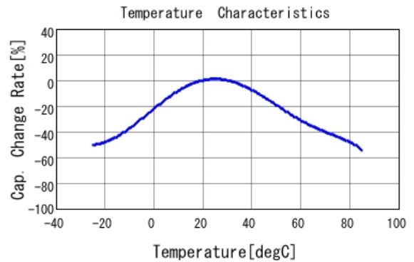
■ DE2E3SA102MA2BT01F C-Temp. capchange, DCOV, AC1Vrms
