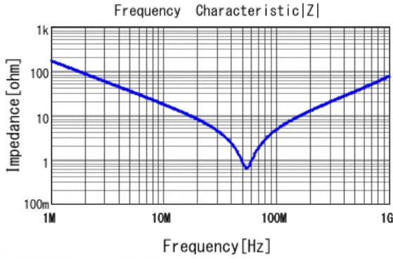
■ DE2E3SA102MA2BT01F |Z| DCOV, 20degC
