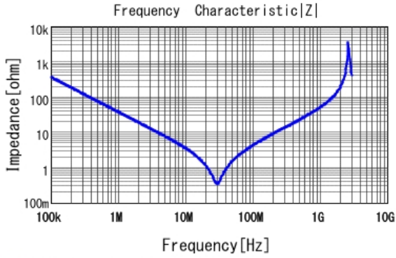
■ DE2E3KY472MN2AM01F |Z| DCOV, 20degC
