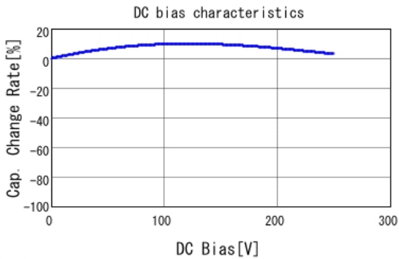
■ DE2E3KY472MN2AM01F C-DC bias capchange, 20.0degC, AC1
