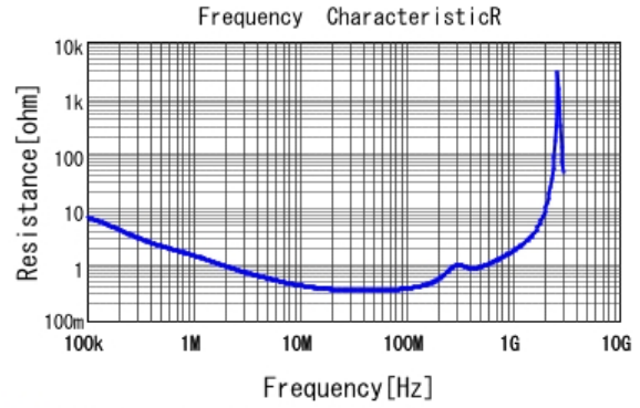
■ DE2E3KY472MN2AM01F R DCOV, 20degC
