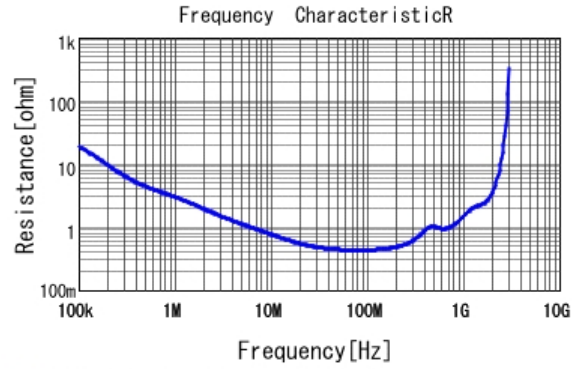
■ DE2E3KY222MN2AM01F R DCOV, 20degC
