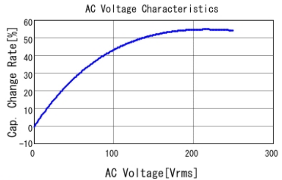
■ DE2E3KY222MN2AM01F C-AC Voltage capchange, DCOV, 20.0
