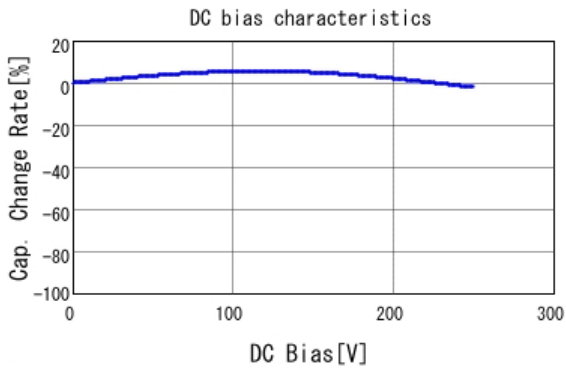
■ DE2E3KY222MN2AM01F C-DC bias capchange, 20.0degC, AC1
