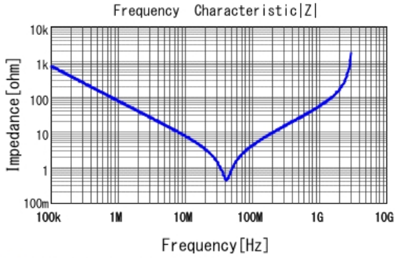
■ DE2E3KY222MN2AM01F |Z| DCOV, 20degC
