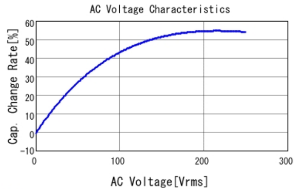
■ DE2E3KY222MB3BM02F C-AC Voltage capchange, DCOV, 20.0
