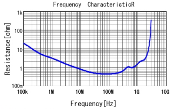
■ DE2E3KY222MB3BM02F R DCOV, 20degC
