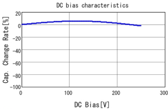
■ DE2E3KY222MB3BM02F C-DC bias capchange, 20.0degC, AC1
