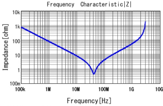
■ DE2E3KY222MB3BM02F |Z| DCOV, 20degC
