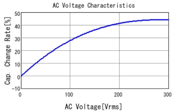
■ DE2E3KY102MN3AU02F C-AC Voltage capchange, DCOV, 20.0
