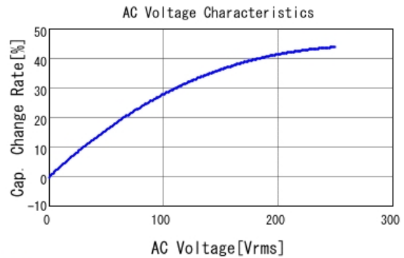
■ DE2E3KY102MB3BM02F C-AC Voltage capchange, DCOV, 20.0
