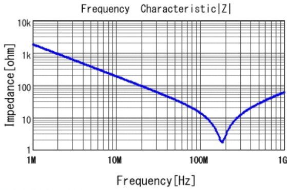
■ DE2B3SA101KN3AX02F |Z| DCOV, 20degC
