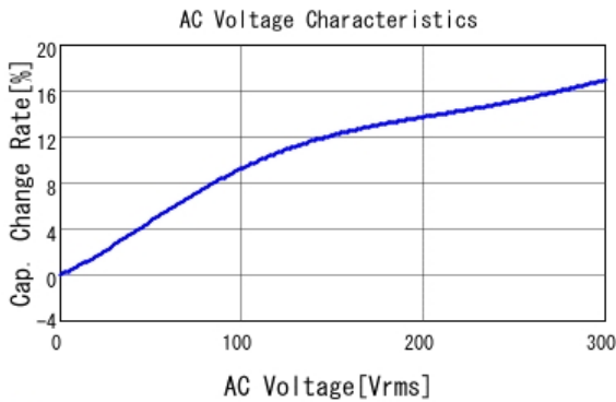
■ DE2B3SA101KN3AX02F C-AC Voltage capchange, DCOV, 20.0
