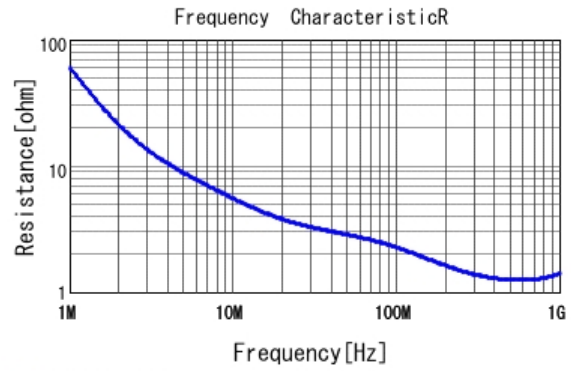
■ DE2B3SA101KN3AX02F R DCOV, 20degC
