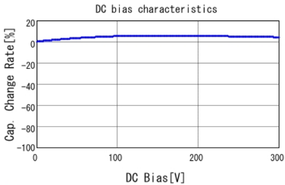
■ DE2B3KY471KA3BU02F C-DC bias capchange, 20.0degC, AC1
