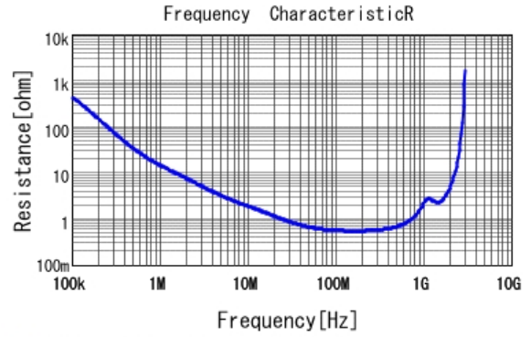
■ DE2B3KY331KN2AM01F R DCOV, 20degC
