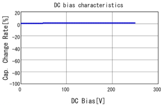
■ DE2B3KY331KN2AM01F C-DC bias capchange, 20.0degC, AC1
