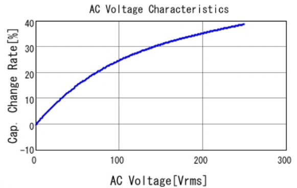
■ DE2B3KY331KN2AM01F C-AC Voltage capchange, DCOV, 20.0
