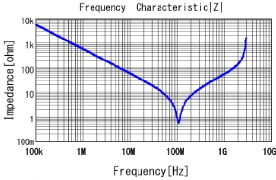
■ DE2B3KY331KN2AM01F |Z| DCOV, 20degC
