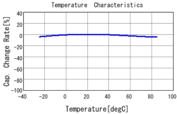
■ DE2B3KY331KN2AM01F C-Temp. capchange, DCOV, AC1Vrms
