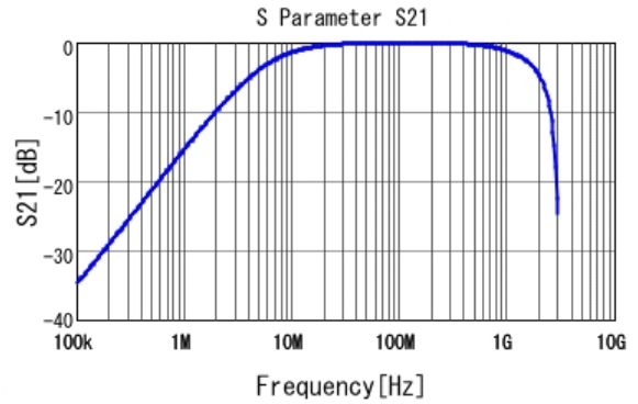
■ DE2B3KY331KN2AM01F S21 DCOV, 20degC
