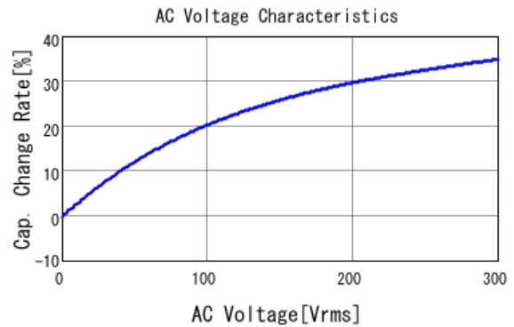
■ DE2B3KY221KA3BU02F C-AC Voltage capchange, DCOV, 20.0
