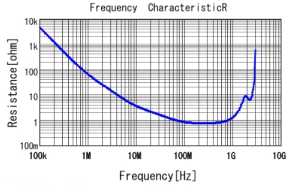
■ DE2B3KY101KN3AM02F R DCOV, 20degC
