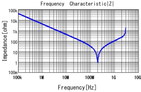
■ DE2B3KY101KN3AM02F |Z| DCOV, 20degC
