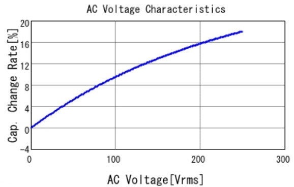
■ DE2B3KY101KN3AM02F C-AC Voltage capchange, DCOV, 20.0
