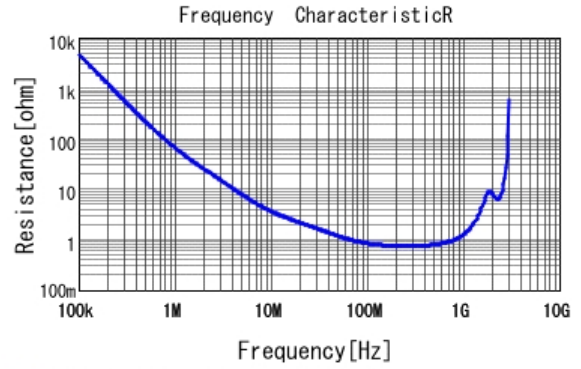
■ DE2B3KY101KN2AM01F R DCOV, 20degC
