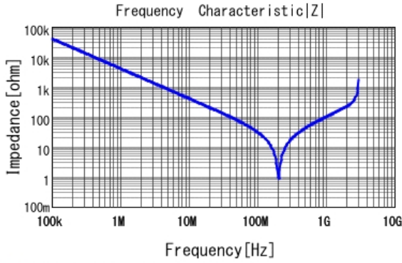
■ DE2B3KY101KN2AM01F |Z| DCOV, 20degC
