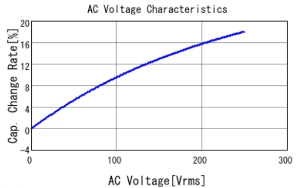
■ DE2B3KY101KN2AM01F C-AC Voltage capchange, DCOV, 20.0
