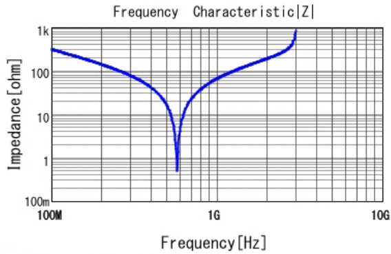
■ DE21XKY100JN2AM01F |Z| DCOV, 20degC
