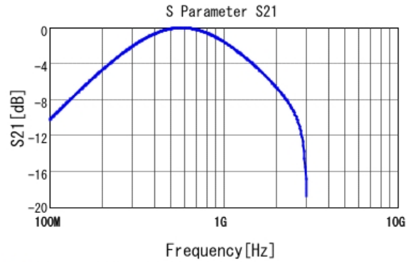
■ DE21XKY100JN2AM01F S21 DCOV, 20degC
