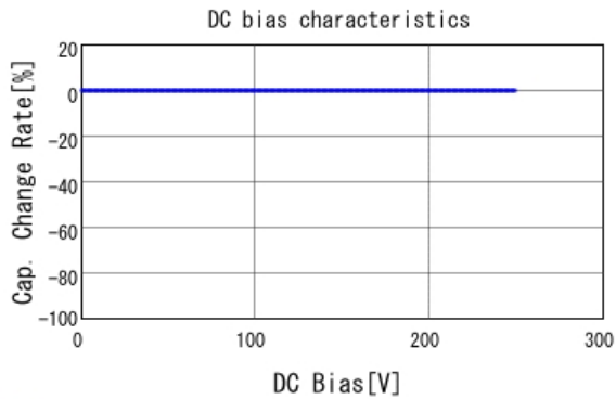
■ DE21XKY100JN2AM01F C-DC bias capchange, 20.0degC, AC1
