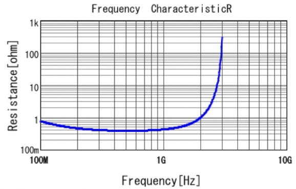
■ DE21XKY100JN2AM01F R DCOV, 20degC
