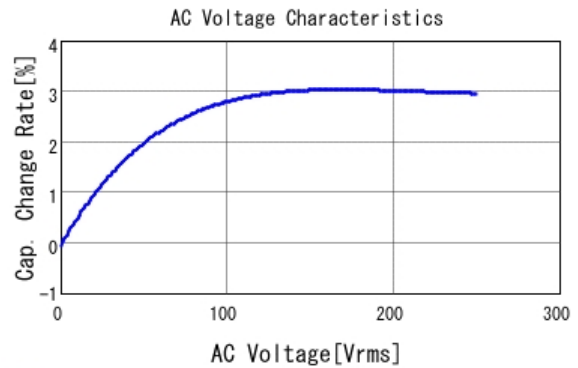
■ DE21XKY100JN2AM01F C-AC Voltage capchange, DCOV, 20.0
