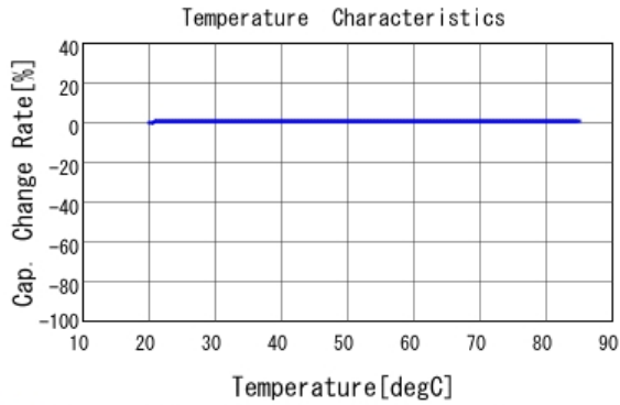
■ DE21XKY100JN2AM01F C-Temp. capchange, DCOV, AC1Vrms
