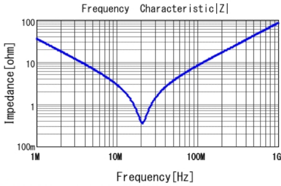
■ DE1E3RA472MJ4BP01F |Z| DCOV, 20degC
