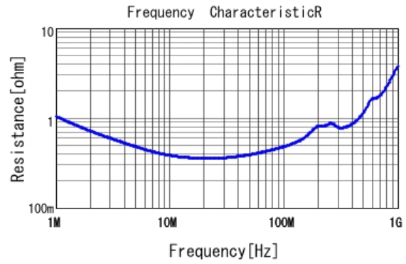
■ DE1E3RA472MJ4BP01F R DCOV, 20degC
