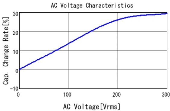
■ DE1E3RA472MJ4BP01F C-AC Voltage capchange, DCOV, 20.0
