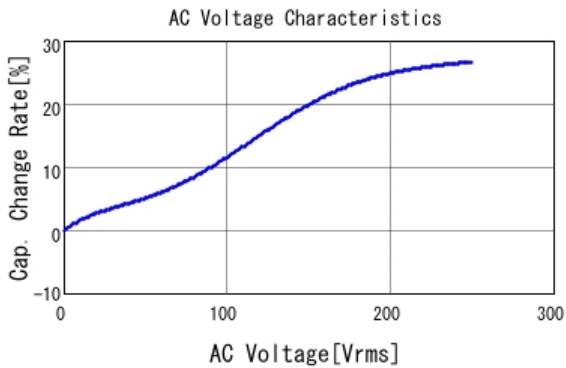
■ DE1E3RA332MA4BN01F C-AC Voltage capchange, DCOV, 20.0
