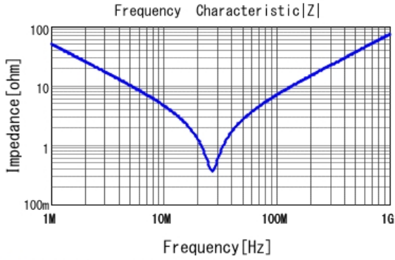
■ DE1E3RA332MA4BN01F |Z| DCOV, 20degC
