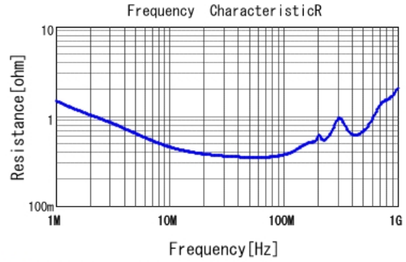
■ DE1E3RA332MA4BN01F R DCOV, 20degC
