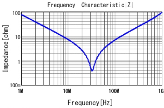
■ DE1E3RA222MN4AP01F |Z| DCOV, 20degC
