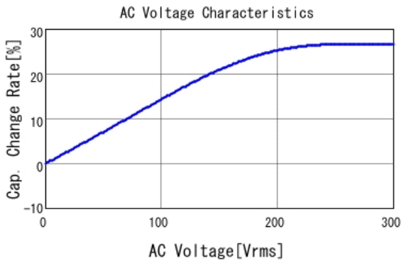
■ DE1E3RA222MN4AP01F C-AC Voltage capchange, DCOV, 20.0
