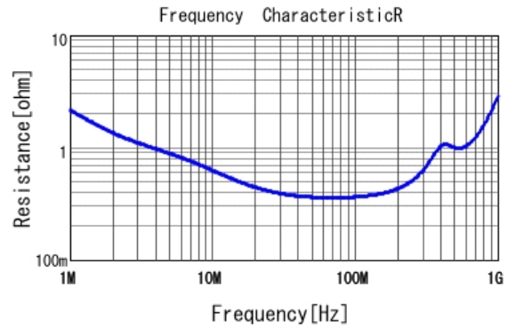
■ DE1E3RA222MN4AP01F R DCOV, 20degC
