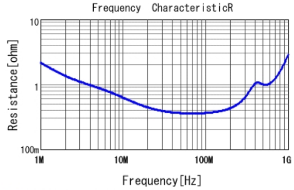
■ DE1E3RA222MA4BP01F R DCOV, 20degC
