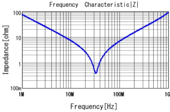
■ DE1E3RA222MA4BP01F |Z| DCOV, 20degC
