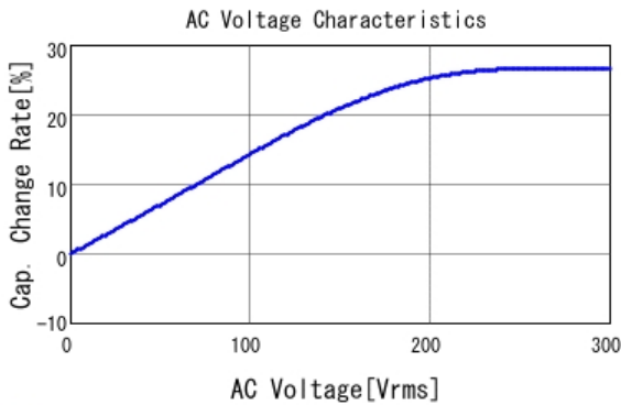
■ DE1E3RA222MA4BP01F C-AC Voltage capchange, DCOV, 20.0
