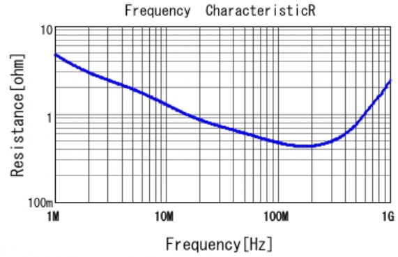
■ DE1E3RA102MA4BP01F R DCOV, 20degC
