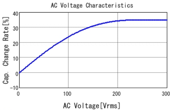
■ DE1E3RA102MA4BP01F C-AC Voltage capchange, DCOV, 20.0
