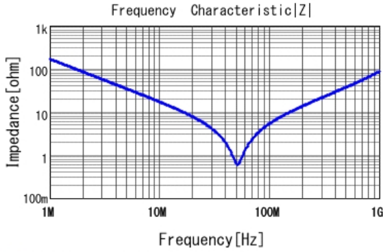
■ DE1E3RA102MA4BP01F |Z| DCOV, 20degC
