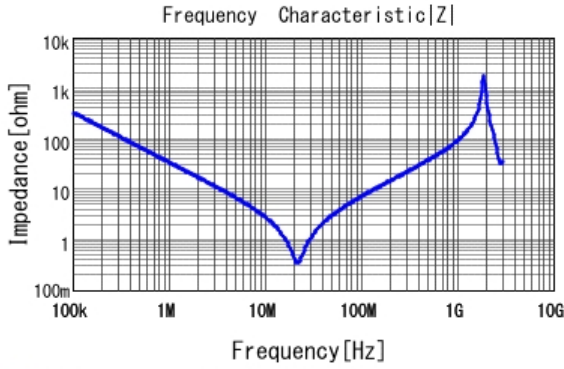
■ DE1E3KX472MN4AP01F |Z| DCOV, 20degC
