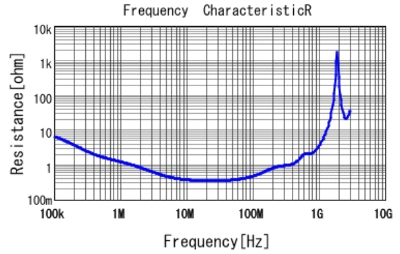
■ DE1E3KX472MA4BP01F R DCOV, 20degC
