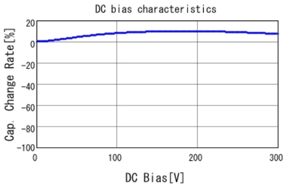
■ DE1E3KX472MA4BP01F C-DC bias capchange, 20.0degC, AC1
