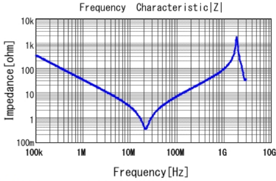
■ DE1E3KX472MA4BP01F |Z| DCOV, 20degC
