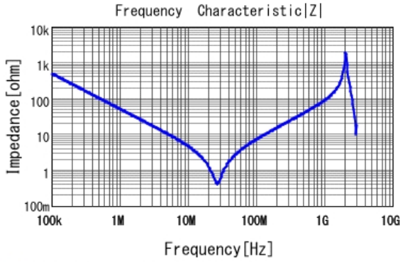
■ DE1E3KX332MN4AP01F |Z| DCOV, 20degC
