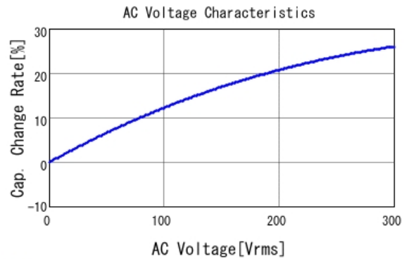
■ DE1E3KX332MN4AP01F C-AC Voltage capchange, DCOV, 20.0
