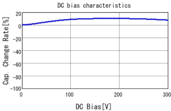
■ DE1E3KX332MN4AP01F C-DC bias capchange, 20.0degC, AC1
