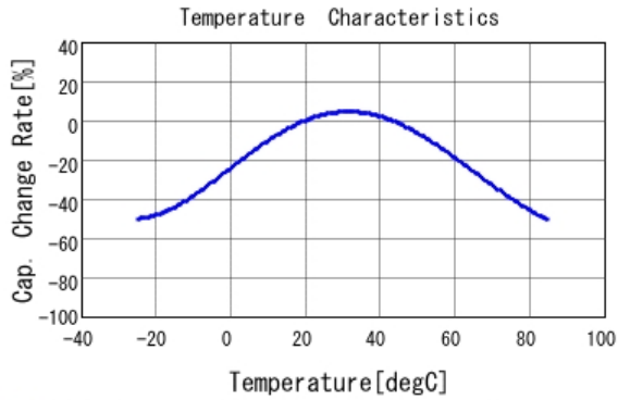
■ DE1E3KX332MN4AP01F C-Temp. capchange, DCOV, AC1Vrms
