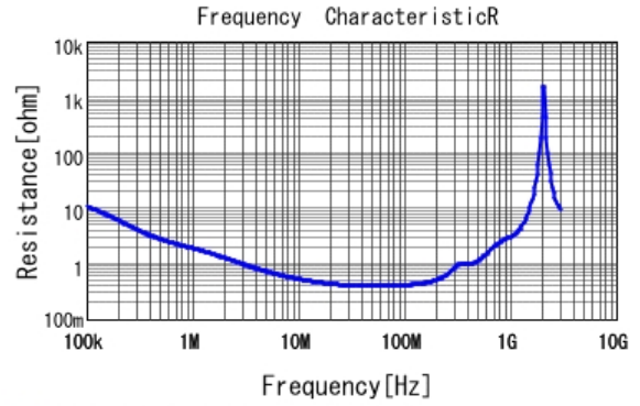
■ DE1E3KX332MB4BP01F R DCOV, 20degC
