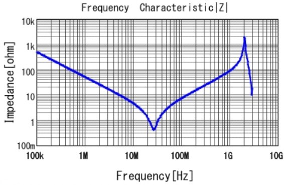
■ DE1E3KX332MB4BP01F |Z| DCOV, 20degC
