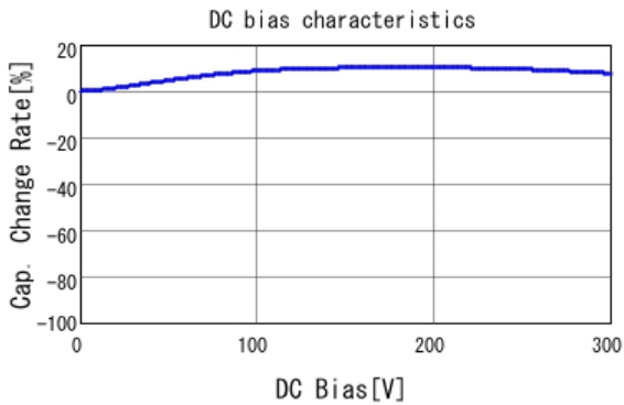
■ DE1E3KX332MB4BP01F C-DC bias capchange, 20.0degC, AC1
