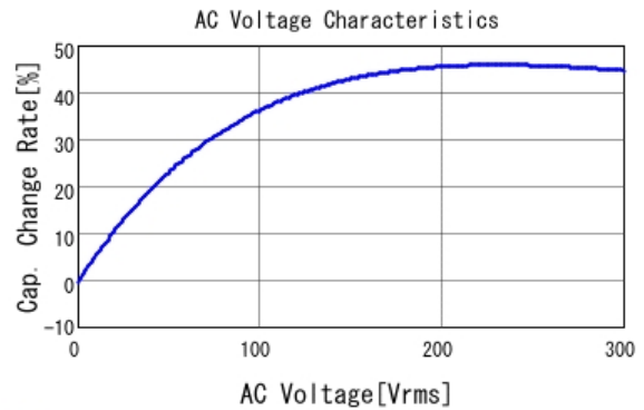
■ DE1E3KX222MA4BP01F C-AC Voltage capchange, DCOV, 20.0
