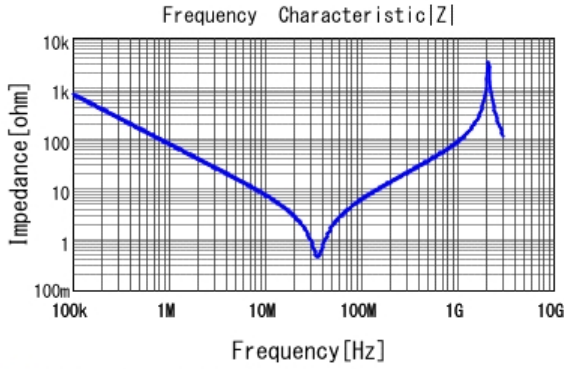
■ DE1E3KX222MA4BP01F |Z| DCOV, 20degC
