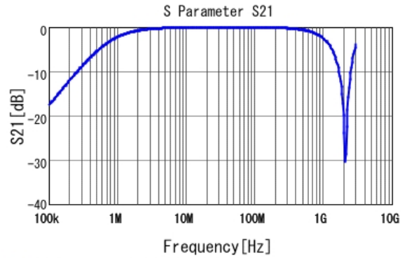
■ DE1E3KX222MA4BP01F S21 DCOV, 20degC
