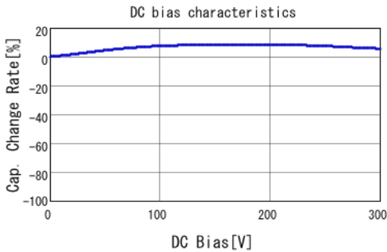
■ DE1E3KX222MA4BP01F C-DC bias capchange, 20.0degC, AC1
