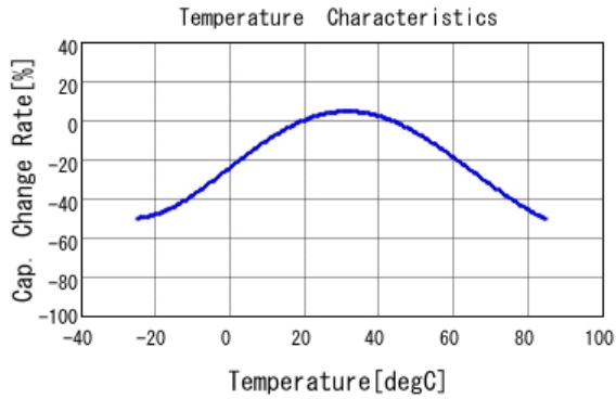
■ DE1E3KX222MA4BP01F C-Temp. capchange, DCOV, AC1Vrms
