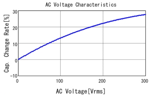
■ DE1E3KX152MN4AP01F C-AC Voltage capchange, DCOV, 20.0
