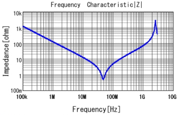
■ DE1E3KX152MN4AP01F |Z| DCOV, 20degC
