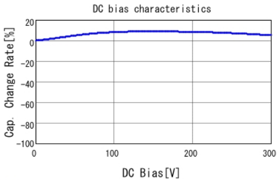
■ DE1E3KX152MN4AP01F C-DC bias capchange, 20.0degC, AC1
